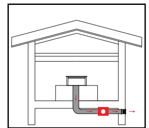
External venting (SEM8 shown)
