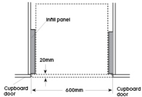
Flush fit top view
