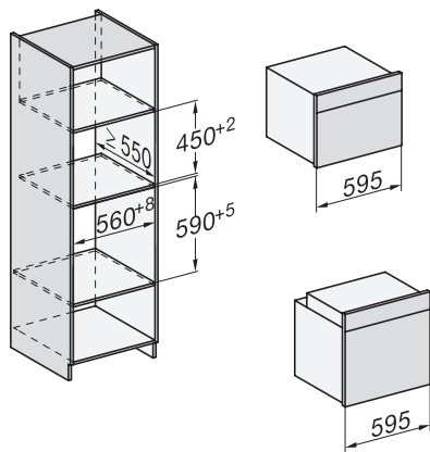
H226x-1B/BP/E/IP, H2760B/BP, H28x0B/BP, H7x40BM/BMX, H7x6x0B/BP/BPX, installation drawings
