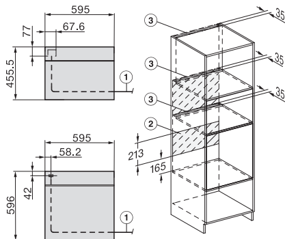
H2xxx-1 B/BP/E/IP, H7xxx B/BP/BM/BMX, installation drawings
