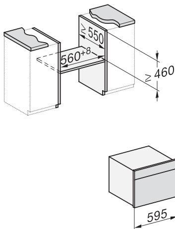
Built-in H 7000 BM build-under, installation drawings
