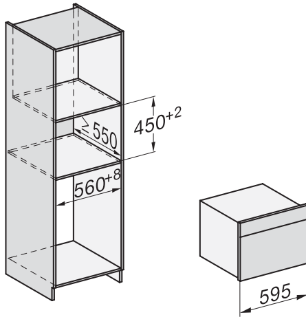
Installation in a tall or base unit
