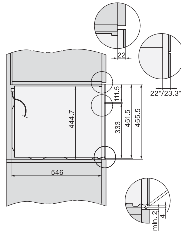
Side view H 7000 BM, 22 mm – glass, 23.3 mm – metal
