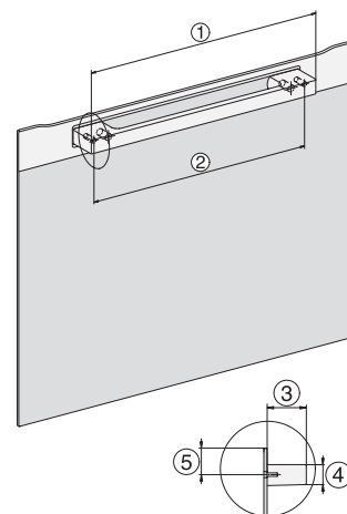
H 7000 handle, installation drawing
